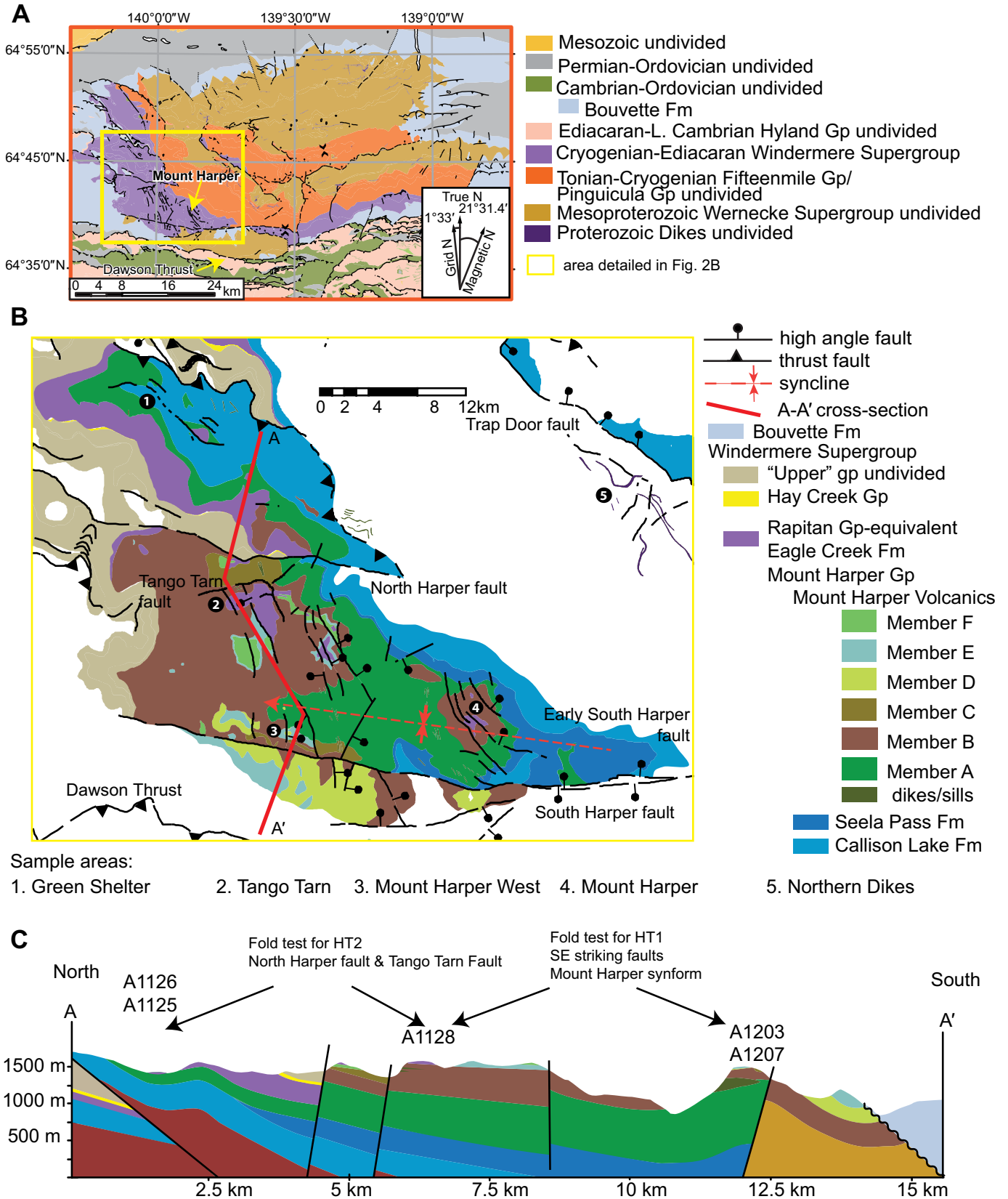
Figure 2. (A) Map of the Coal Creek inlier (modified from Strauss et al., 2014b). (B) Focus on the Mount Harper Group with the Mount Harper volcanics divided into informal members. Important sample areas and cross-section line A-A' are indicated on map. (C) Cross-section A-A' across the Mount Harper volcanics.
