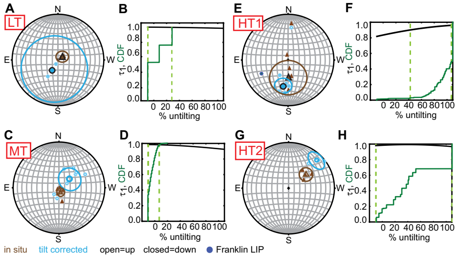
Figure 5. (A) Sections with a low-temperature (LT) direction. (B) Results from the Tauxe and Watson (1994) fold test. (C) Sections with a mid-temperature (MT) direction. (D) Results from the Tauxe and Watson (1994) fold test. (E) Section results for the first high-temperature (HT1) direction. Note that site A1207 has a high stability HT1 direction reversed from the rest. The direction expected from the Franklin large igneous province (LIP; Denyszyn et al., 2009a) is also indicated. (F) Results for HT1 from the Tauxe and Watson (1994) fold test. (G) Section results for the second high-temperature (HT2) direction. (H) Results for HT2 from the Tauxe and Watson (1994) fold test. For the plots of the section-mean directions, the in situ directions are indicated with brown triangles, and the tilt-corrected directions are indicated with blue circles, with negative directions represented by open symbols and positive directions represented by closed symbols. For the Tauxe and Watson (1994) fold tests, the black curves indicate maximum eigenvalue ( \tau_1 ) as a function of untilting. The green line is the cumulative distribution of the percent untilting required to maximize \tau_1 for all the bootstrapped data sets. The dashed vertical lines are 95% confidence bounds on the percent untilting that yield the most clustered result (maximum \tau_1 ). If the 95% confidence bounds include 0, then a pretilt magnetization is indicated. If the 95% confidence bounds include 100, then a post-tilt magnetization is indicated. If the 95% confidence bounds exclude both 0 and 100, syntilt magnetization is possible. CDF—cumulative distribution function.
