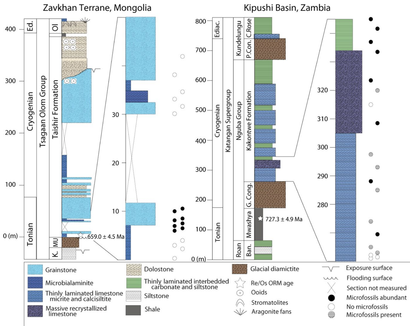
FIGURE 1 Stratigraphic columns of the Tsagaan Olom Group of the Zavkhan Terrane, Mongolia, (a) and the Katangan Supergroup of the Kipushi Basin, Zambia (b). Columns show the stratigraphic location of the Taishir Formation (a) and the Kakontwe Formation (b) with the location of samples and microfossil occurrence
