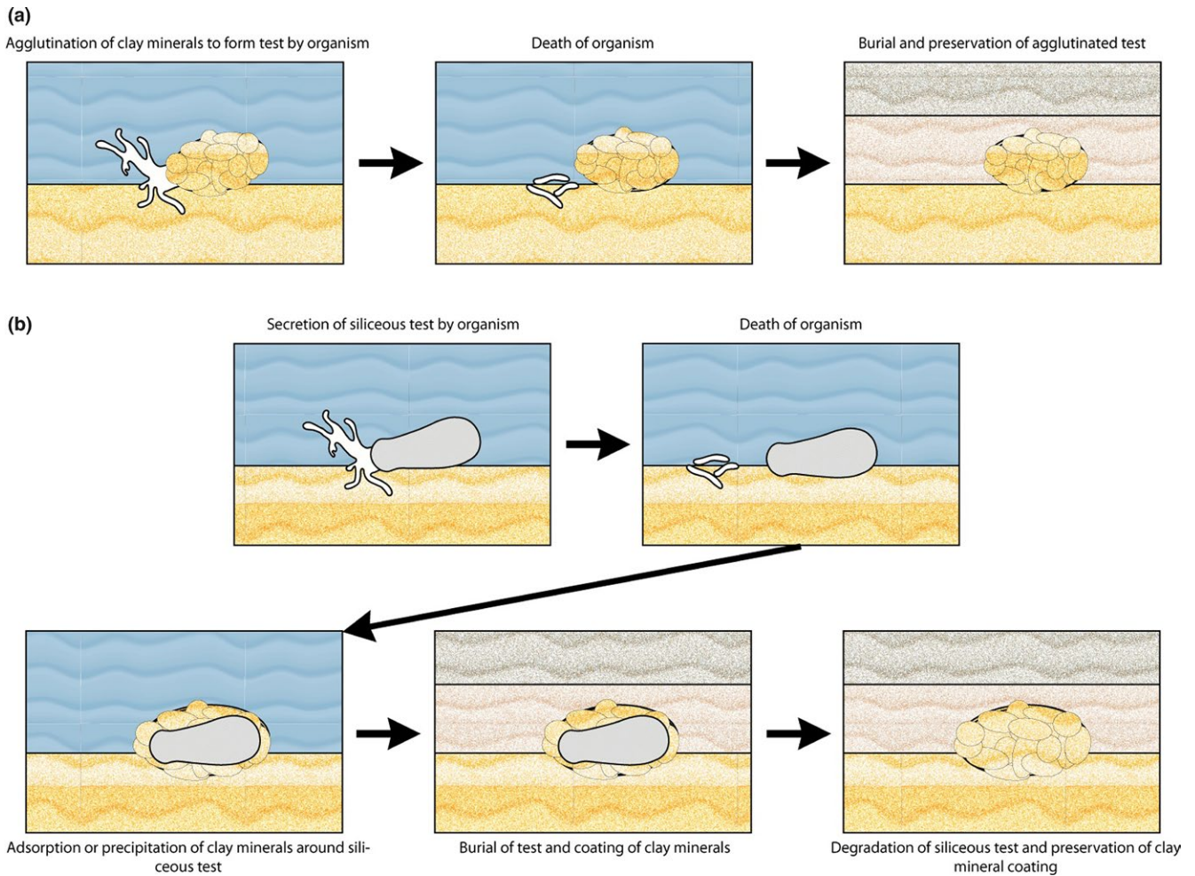
FIGURE 10 Cartoon depictions of possible preservation models for microfossils of the Kakontwe, Taishir and Rasthof formations. Model “a” illustrates preservation of an originally agglutinated test. Model “b” depicts diagenetic alteration through adsorption or precipitation of clay minerals to an originally siliceous or organic-walled test.
