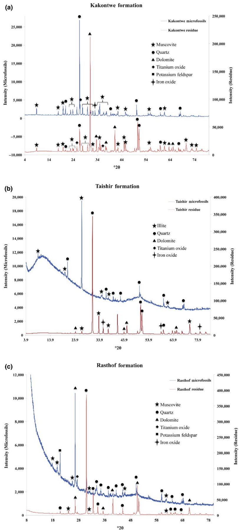
FIGURE 9 XRD spectra showing mineralogy of putative microfossils (blue) and residues (red) from the Kakontwe (a), Taishir (b) and Rasthof (c) formations. Residues and putative microfossils from all three localities have the same composition and contain illite or muscovite as the major clay mineral
