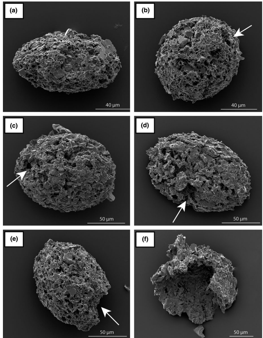
FIGURE 5 SEM images of putative microfossils from the Rasthof Formation. Structures show characteristic morphologies, including elongated ovoid forms (a), spherical forms with possible openings shown by a white arrow (b), ovoid forms with possible openings shown by arrows (c, d), structures with hoods shown by an arrow (e) and broken forms showing a hollow interior with 10 \pm 1 \mu\text{m} -thick walls (f)
