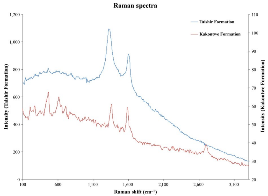
FIGURE 7 Raman spectrometry data showing peaks at \sim 1320 to 1360 \text{ cm}^{-1} and \sim 1590 \text{ cm}^{-1} characteristic of carbonaceous material in the walls of putative microfossils
