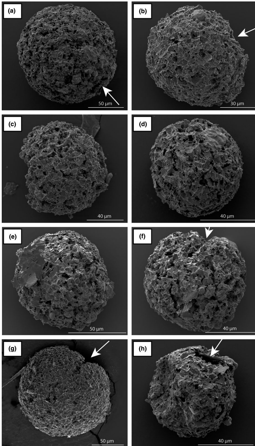
FIGURE 4 SEM images of characteristic structures from the Taishir Formation. Structures are predominantly spherical with possible openings highlighted by white arrows (a, h), concave (b, c) or blunt (d, e) edges, possible elongated openings indicated by arrows (f, g) or tapering along the long axis (e). Structures are hollow and have 10 \pm 1 \mu\text{m} -thick walls (h)
