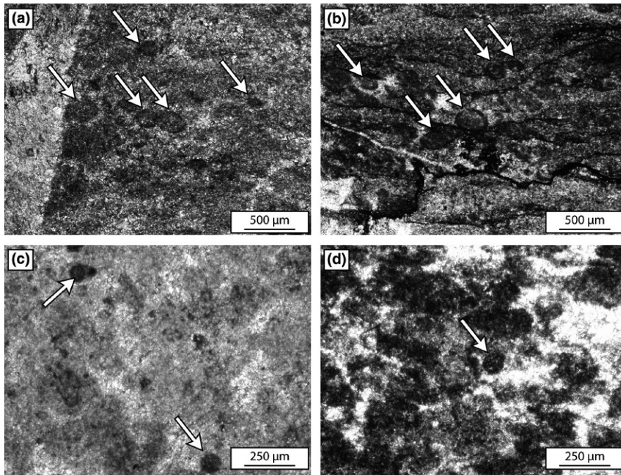
FIGURE 6 Petrographic thin section images of samples from the Kakontwe (a, b) and Taishir (c, d) formations. Putative microfossils from the Kakontwe Formation are found in both unlaminated (a) and microbially laminated (b) limestones. These structures are oval to circular in thin section and have a distinct outer wall with micritic filling. Putative microfossils from the Taishir Formation are found in unlaminated limestones and are circular in thin section and infilled with dark micrite (c, d)
