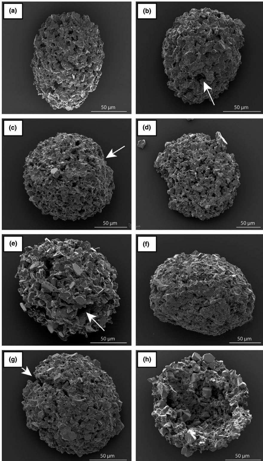
FIGURE 2 SEM images of putative microfossils from the Kakontwe Formation. Structures demonstrate ovoid morphologies that taper along the long axis to create a tear shape (a), ovoid tapering morphologies with possible openings shown by a white arrow (b), spherical morphologies with blunt (c) or concave (d) edges (highlighted by a white arrow), ovoid morphologies with possible opening along the smaller axis shown by a white arrow (e), ovoid morphologies with blunt edges (f), ovoid morphologies with possible breaks shown by an arrow (g) and broken specimens demonstrating a hollow interior with 10 \pm 1 - \mu\text{m} -thick walls (h)
