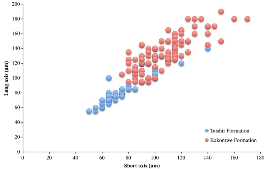
FIGURE 3 Size distributions of the long and short axes of putative microfossils from the Kakontwe and Taishir formations. Structures of the Kakontwe Formation and the Taishir Formation both demonstrate a normal distribution. Structures from the Kakontwe Formation have slightly larger sizes than those of the Taishir Formation, although the ranges for the two formations have clear overlap
