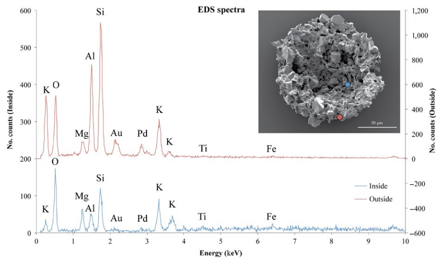
FIGURE 8 EDS data showing the elemental compositions of the interior and exterior surfaces of microfossils. Au and Pd peaks are the result of gold and palladium coating used on samples to enhance conductivity and are not originally present in samples
